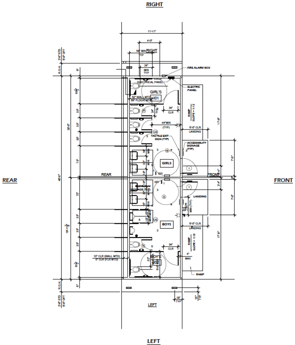
FLOOR PLAN 12'X40' TOILET A (BOY/GIRL) TYPICAL RESTROOM
