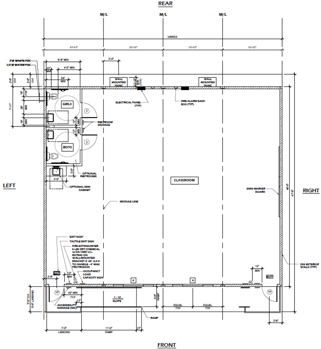
FLOOR PLAN 48'X40' TYPICAL CLASSROOM
