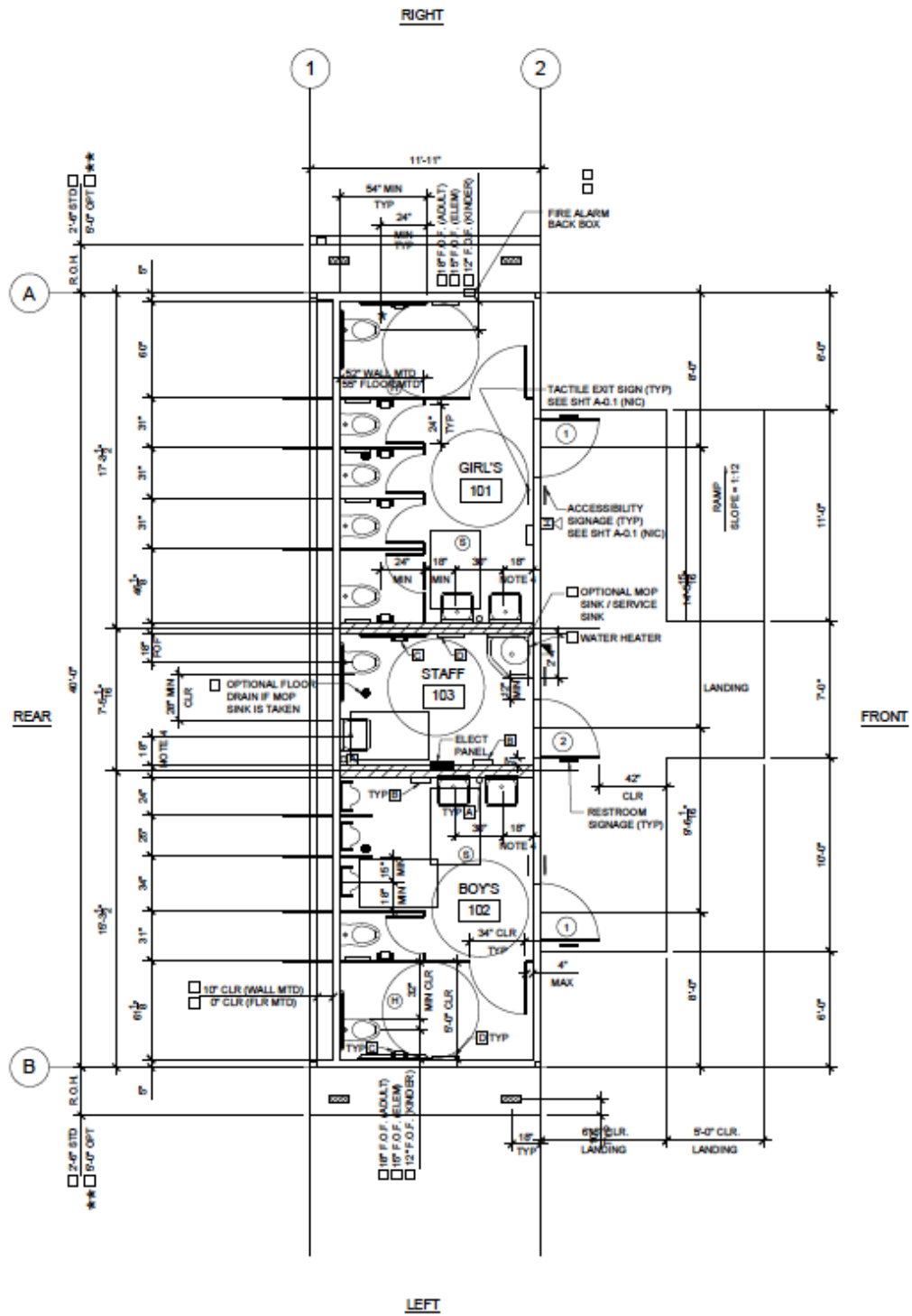
FLOOR PLAN 12'X40' TOILET B (BOY/STAFF/GIRL) TYPICAL RESTROOM
