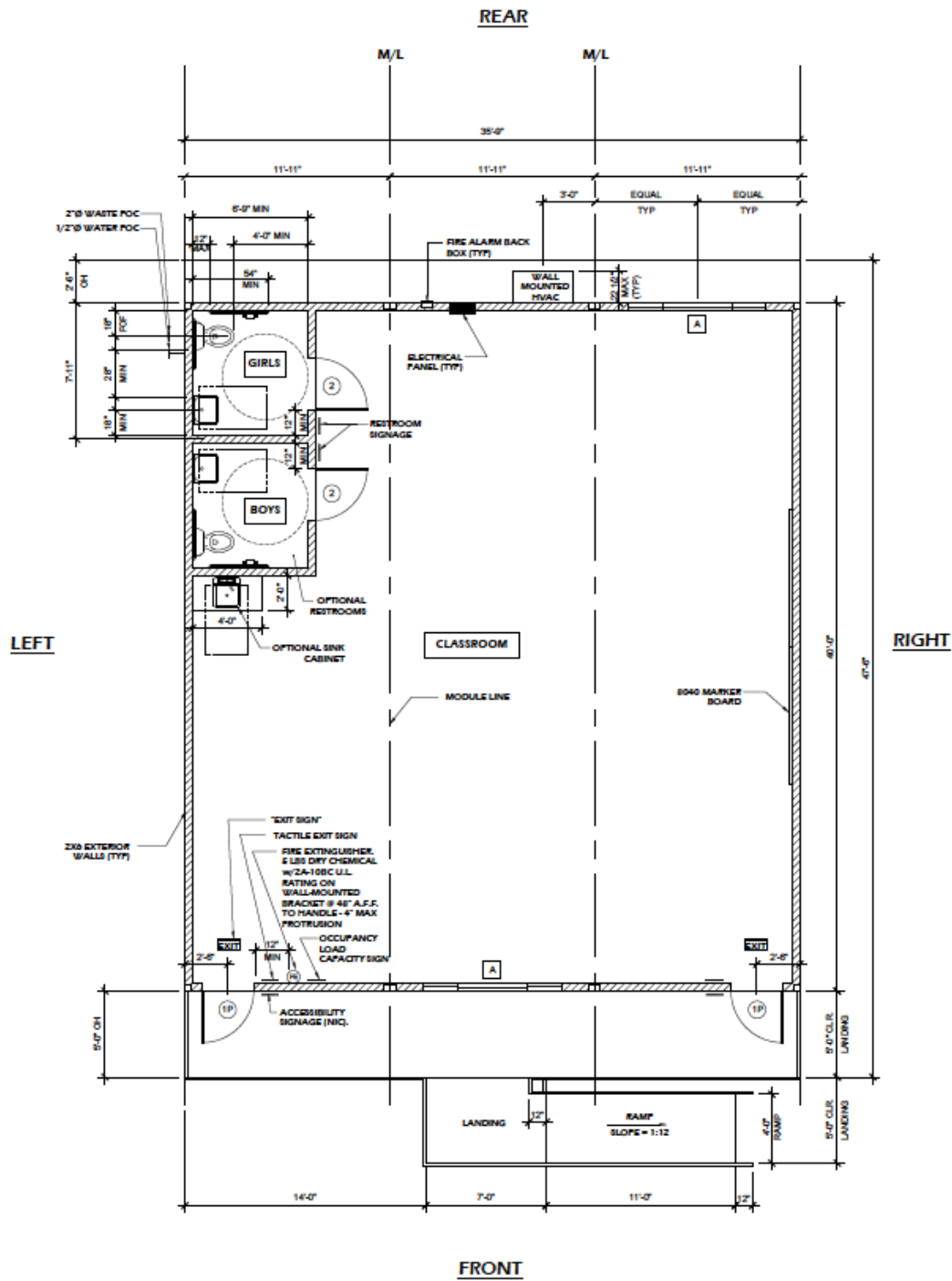
FLOOR PLAN 36'X40' TYPICAL CLASSROOM
