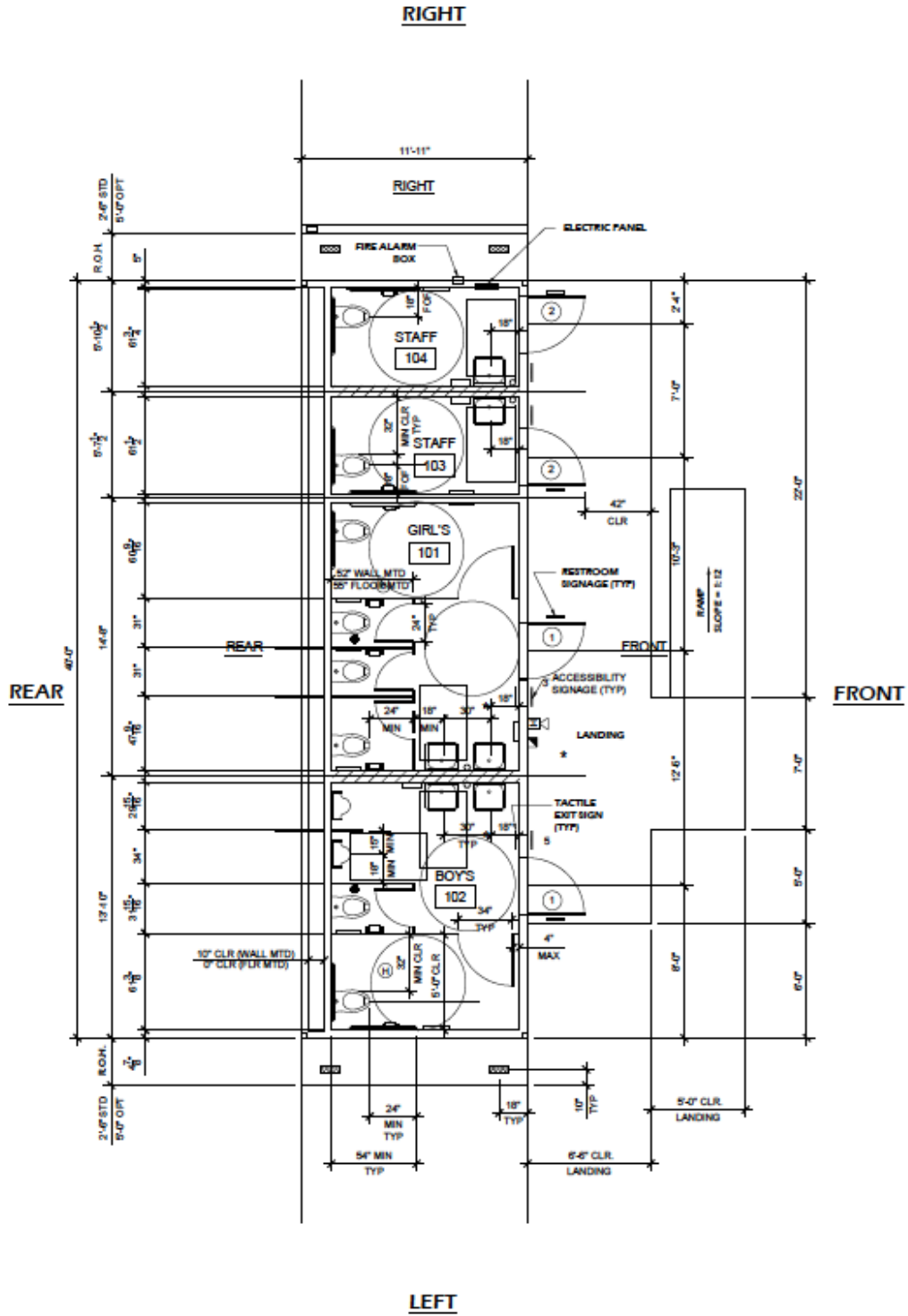
FLOOR PLAN 12'X40' TOILET C (BOY/GIRL/STAFF/STAFF) TYPICAL RESTROOM
